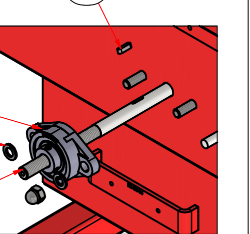
B Detail (Scale 1 : 4)
