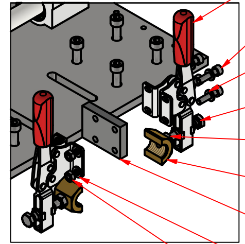
F Detail (Scale 1 : 4 )
