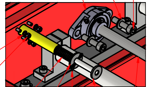
E Detail (Scale 1 : 4 )
